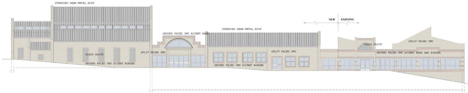
4 WEST ELEVATION A-201 3/32"=1'-0"
