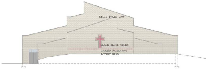
2 NORTH ELEVATION A-201 3/32"=1'-0"
