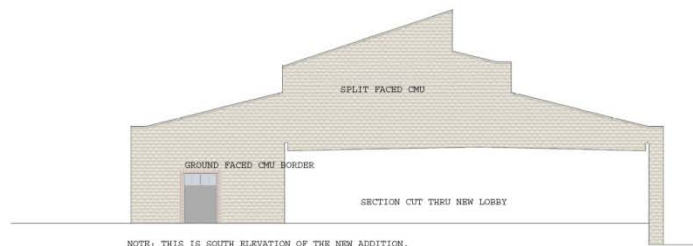
3 SOUTH ELEVATION A-201 3/32"=1'-0"
