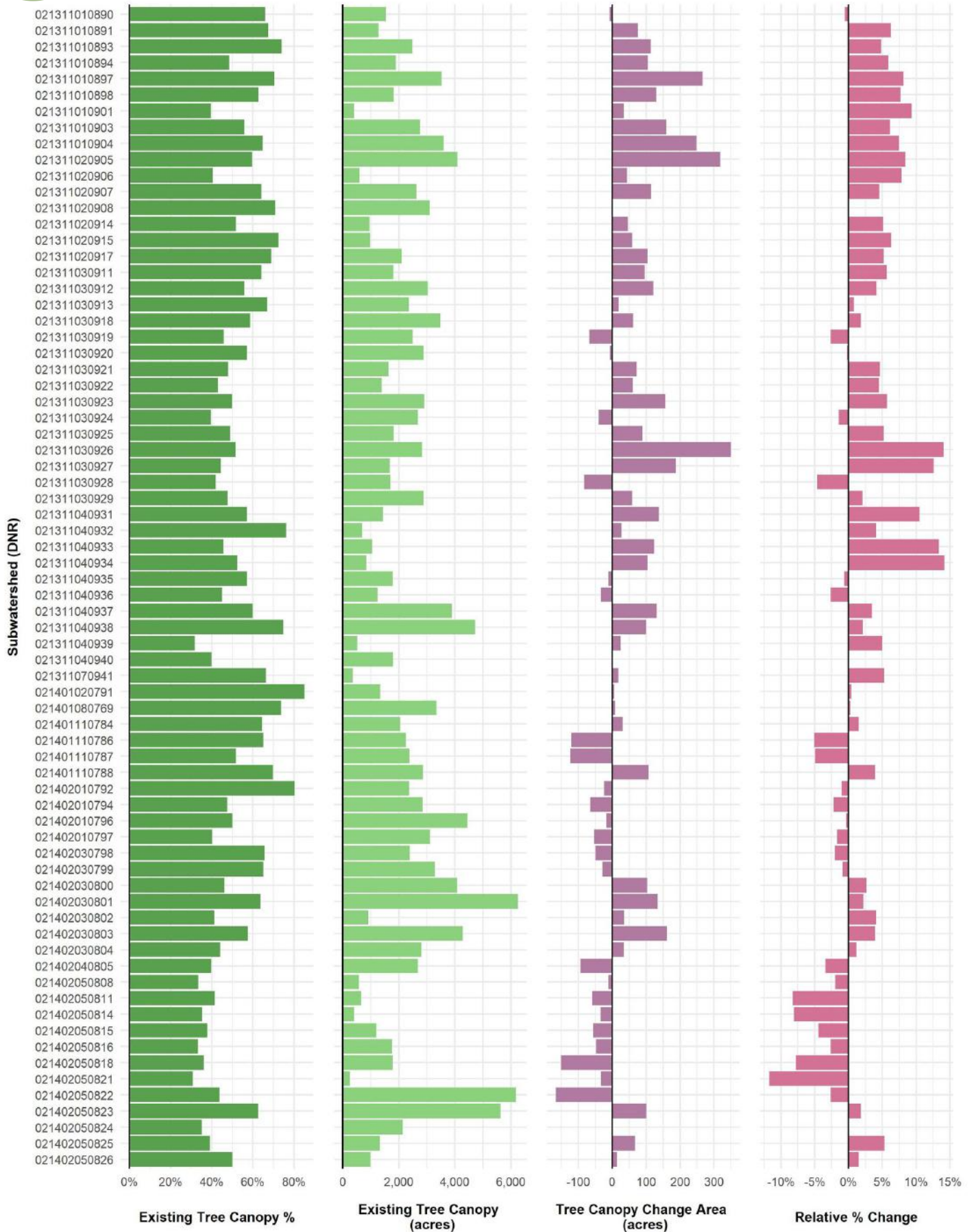
Figure 26: Tree canopy and change metrics summarized by subwatershed.
