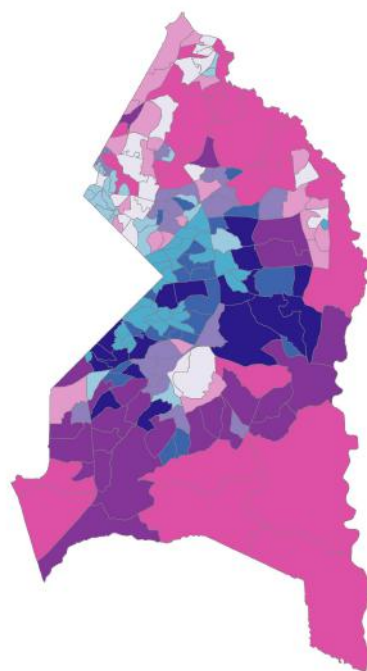
Figure 27: These maps show percent existing tree canopy cover in relation to two demographic groups that are highly interrelated and typically within the most susceptible groups against environmental challenges. Shades of pink indicate tree canopy percentage by block group, with the darkest shade indicating higher percentages. Meanwhile, shades of blue indicate percentage of residents within each of the demographic groups, with the darkest shade indicating higher percentages.
