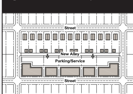
Figure 8.28c Rear Alley Access
