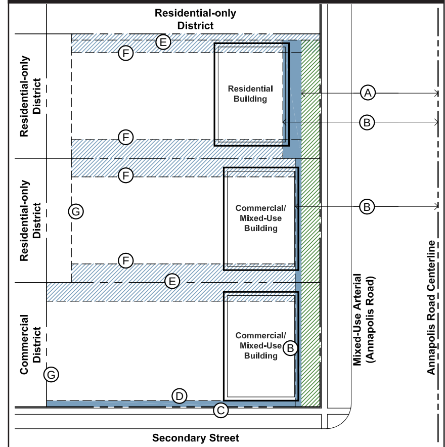
Figure 8.20a Mixed-use Arterial Bulk Diagram
