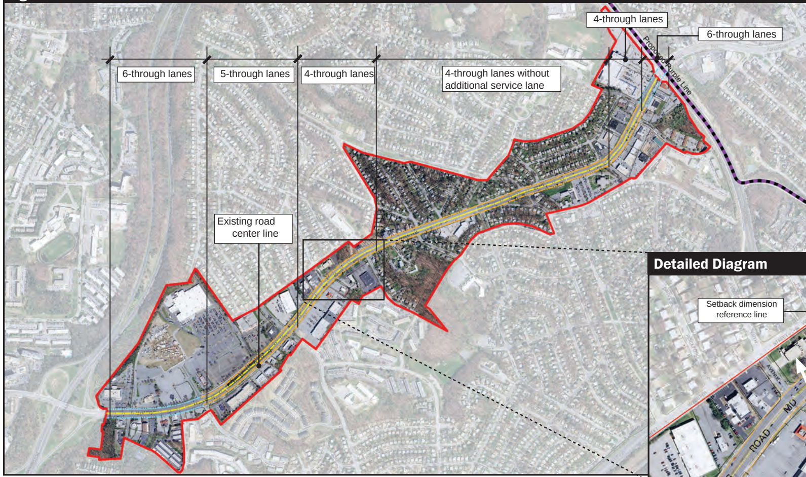
Figure 8.9 Setback Reference Line
