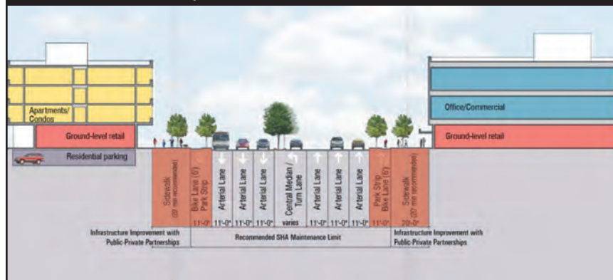
Section 6-a: Cross section of Annapolis Road between Veterans Parkway and Gallatin Street
