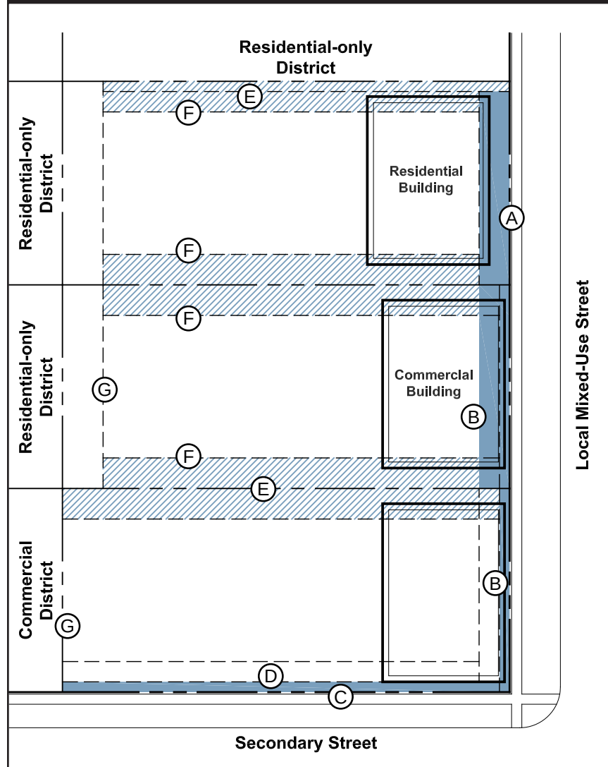
Figure 8.20b Local Mixed-use Street Bulk Diagram
